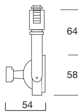
Gimbal Ring MR16
