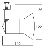
Rocket with Cone PAR30
