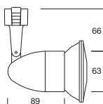
T3425/S LumaPAR Ellipse 1-circuit track adaptor WH SG BL
