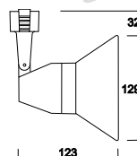
T3230/S LumaPAR Flat-Back with cone 1-circuit track adaptor WH SG BL
