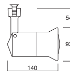
Rocket with Cone R60 / R63 / PAR20
