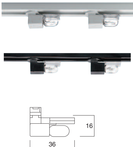
Xenon Bud
