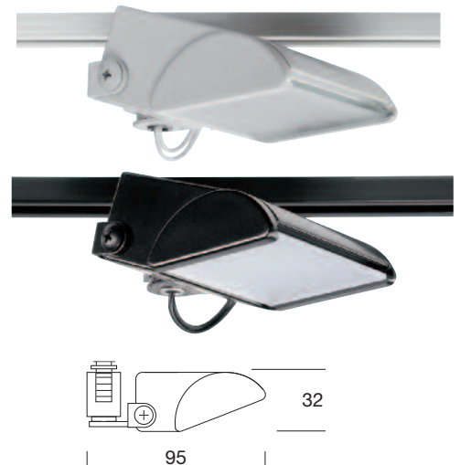
Halogen Flood
