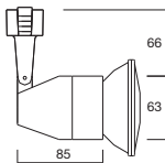
T3225/S LumaPAR Flat-Back 1-circuit track adaptor WH SG BL
