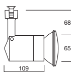
Rocket PAR30
