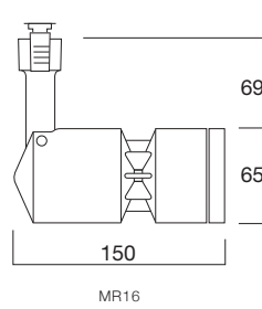
MR16
